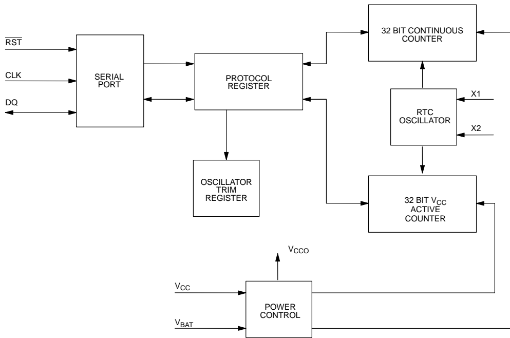
DS1602 ELAPSED TIME COUNTER BLOCK DIAGRAM Figure 1
